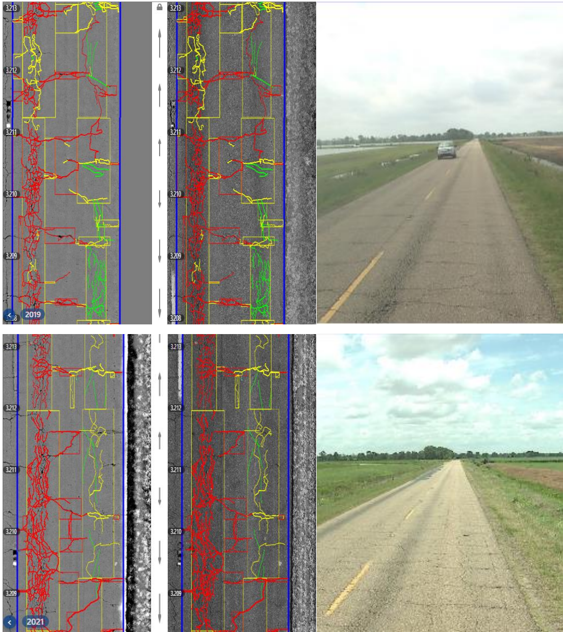
Figure 36. Pavement images and rut index profiles for CS849-10
