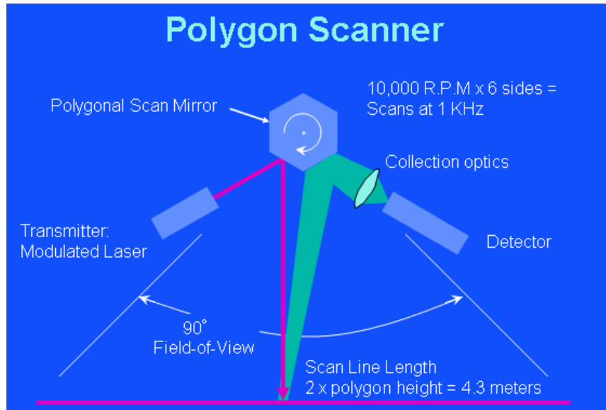
Figure 9. Polygon scanner [10]
