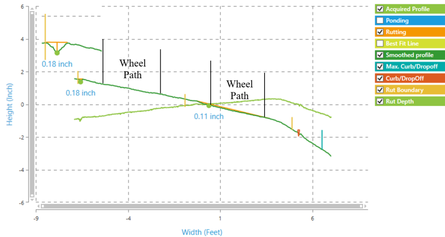
Figure 26. Measurement outside the wheel path for Fugro's full profile rut depth
