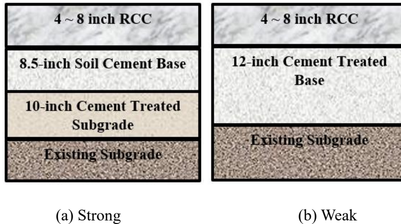
Figure 14. RCC pavement structure
