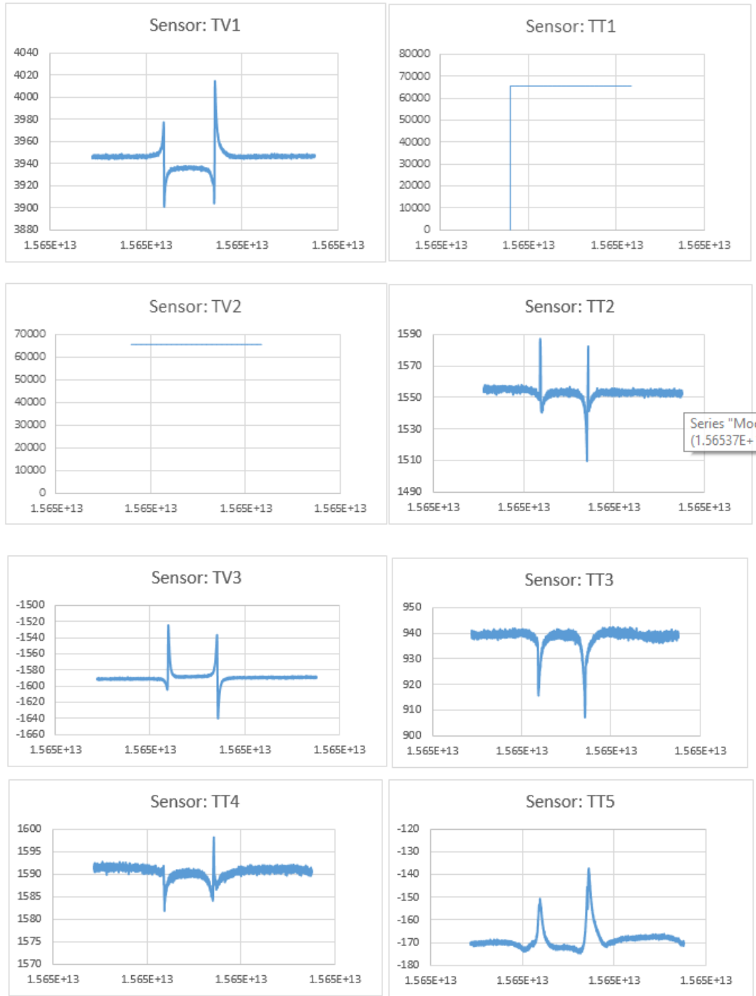
Figure A5. Dynamic top strain response at 9-kip loading (section 4)
