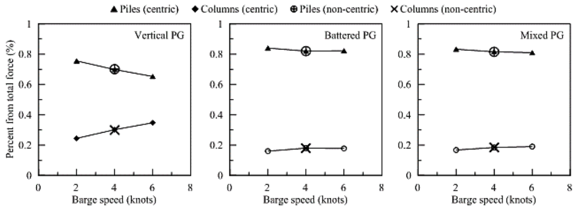
Figure 179. Contribution of piles and pier columns to the resisting force in centric and non-centric impacts
