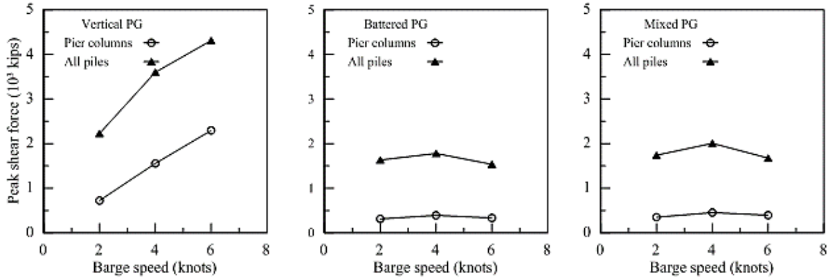
Figure 172. Results of peak shear versus barge speed
