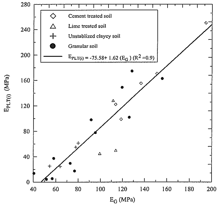
Figure 67 Correlation between E_G and the E_{PLT(i)} (field test)
