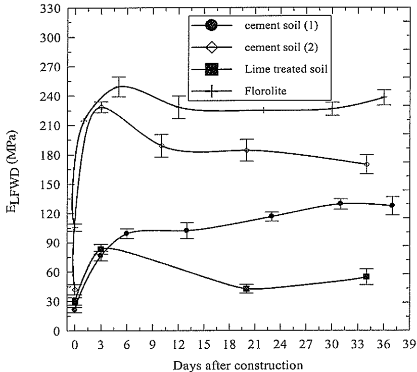
Figure 54 E_{LFWD} variation with time
