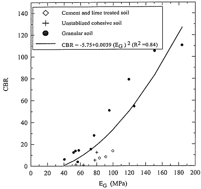
Figure 73 Correlation between E_G and CBR (field test)
