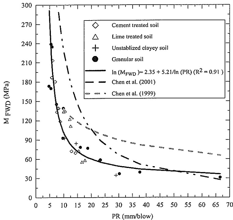
Figure 89 Correlation between DCP- PR and M_{FWD}
