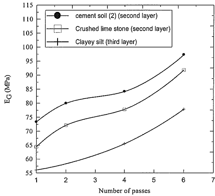
Figure 50 Geogauge modulus variation with number of passes
