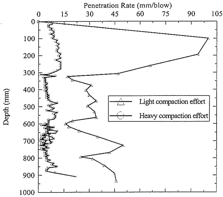
Figure 62 DCP-PR profiles for RAP trench sections
