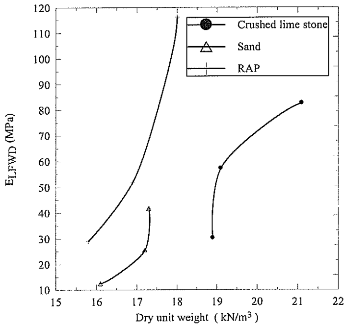
Figure 60 E LFWWD and dry unit weight for different trenches
