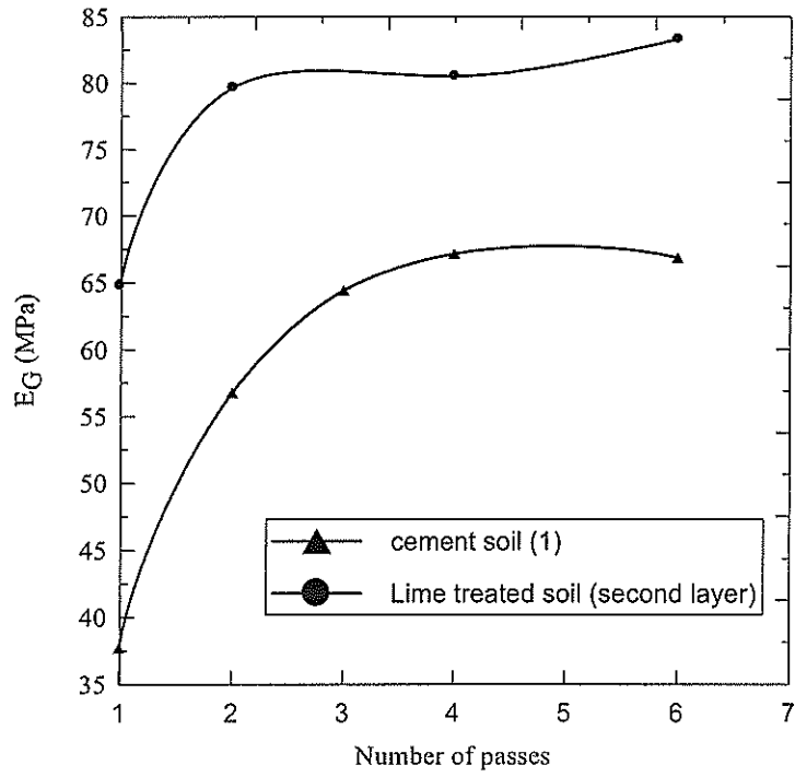
Figure 49 Geogauge modulus variation with number of passes
