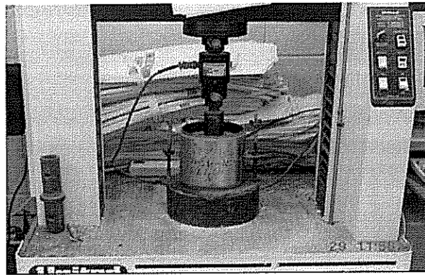
Figure 38 United machine used to conduct CBR test
