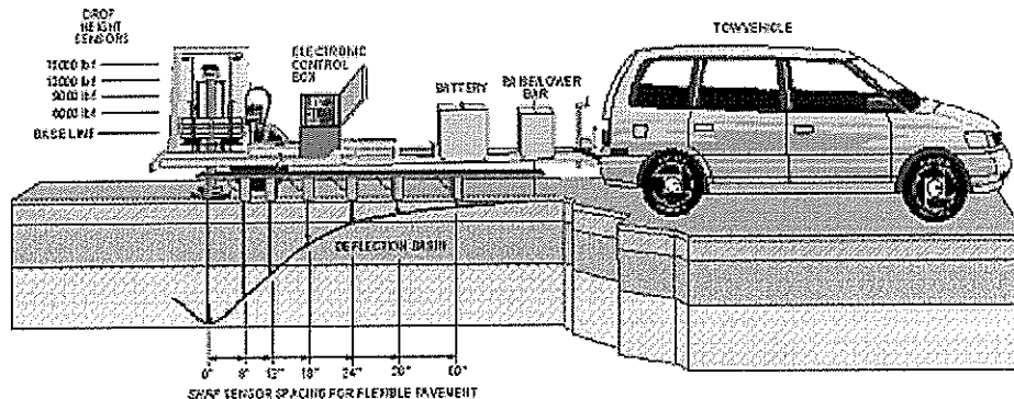
Figure 5 Dynatest model 8000 (FWD) (LTRC 2000)
