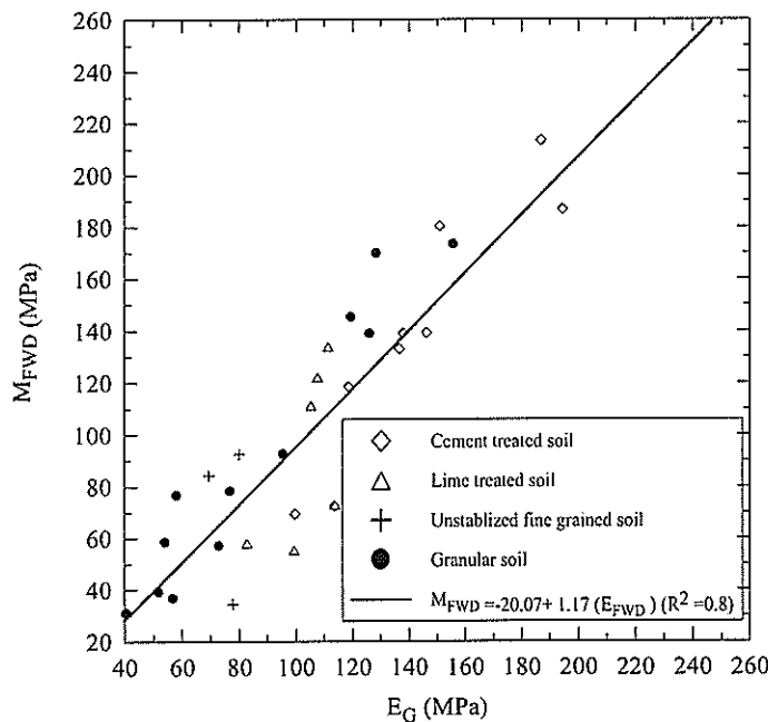
Figure 71 Correlation between E_G and the M_{FWD}
