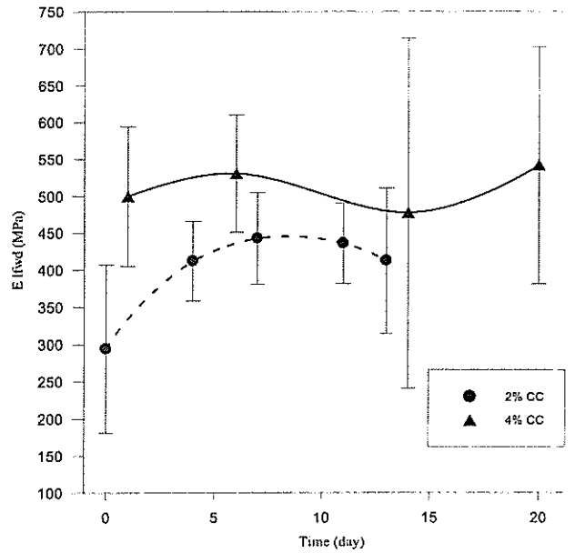
Figure 41 E_{LFWD} with time for cement-soil
