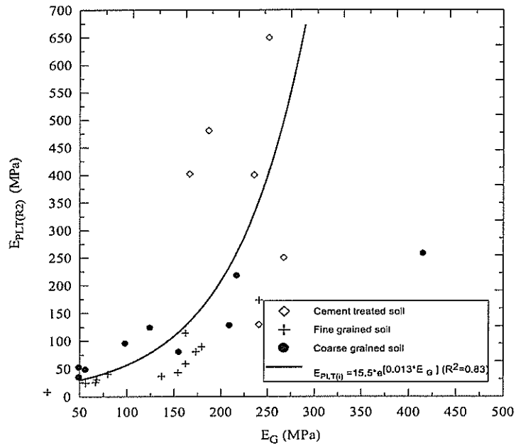
Figure 65 Correlation between E_G and the E_{PLT(i)} (laboratory test)
