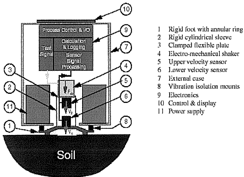
Figure A1 Schematic of the Geogauge (Humboldt, 1998)
