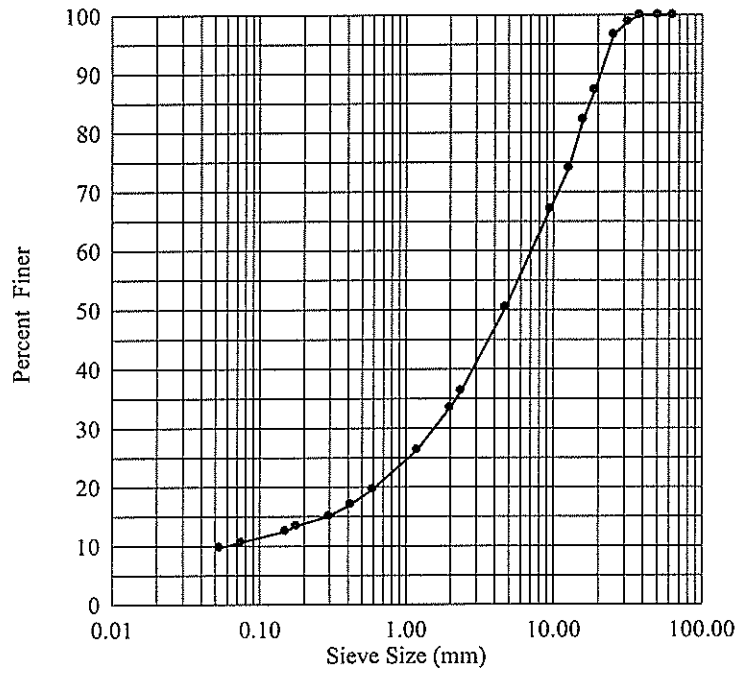
Figure 35 Gradation of crushed limestone
