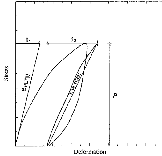
Figure 6 Definition of modulus from PLT
