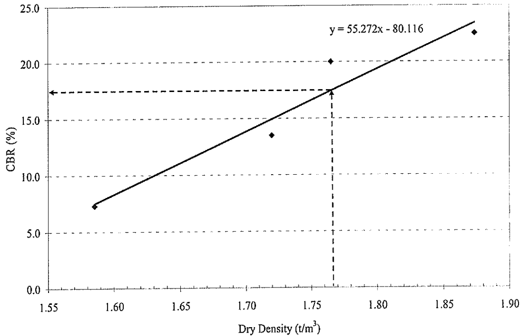
Figure 17 Determination of CBR for desired dry unit weight
