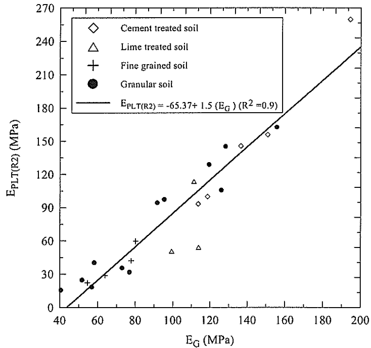
Figure 68 Correlation between E_G and the E_{PLT(R2)} (field test)
