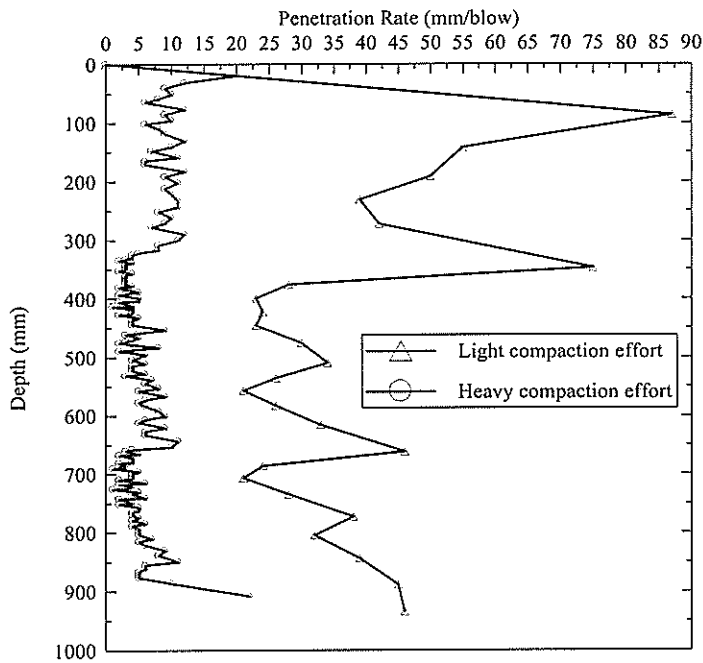
Figure 61 DCP-PR profiles for crushed limestone trench sections
