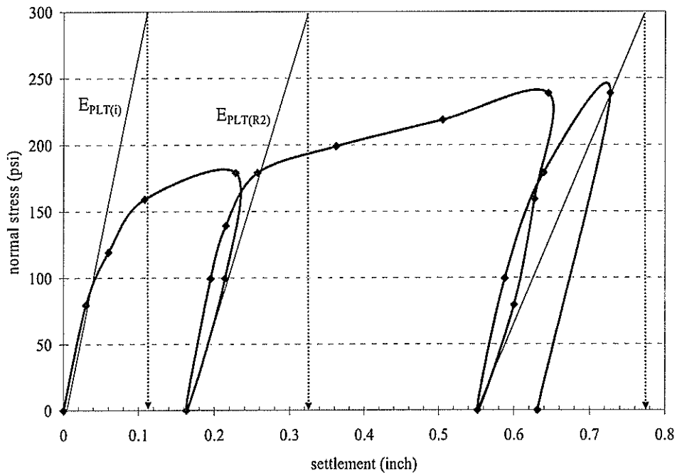
Figure 16 Typical Plate Load Test results
