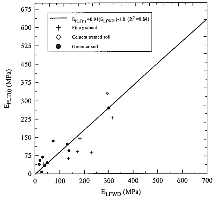
Figure 74 Correlation between E_{LFWD} and the E_{PLT(i)} (laboratory test)
