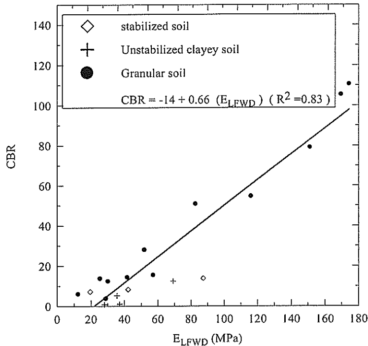
Figure 82 Correlation between ( E_{LFWD} ) and CBR (%) (field test)
