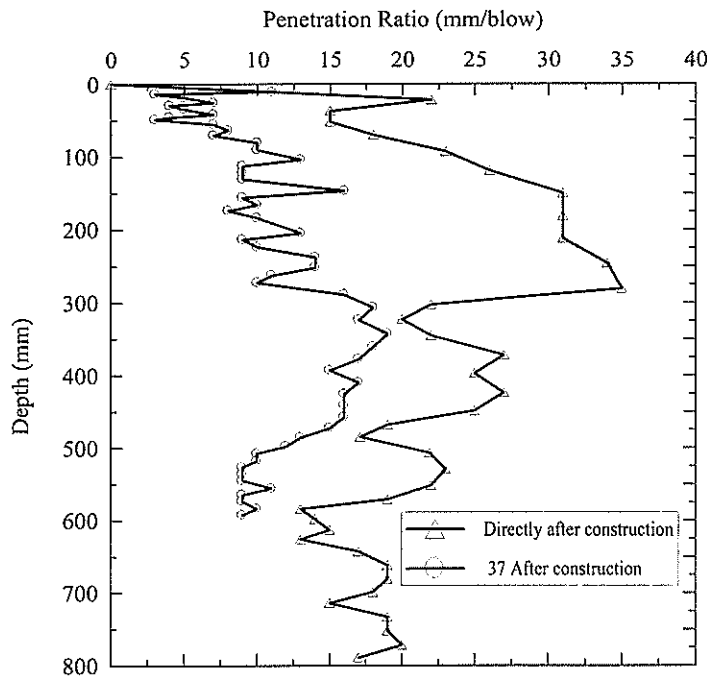
Figure 55 DCP-PR with time for cement soil section (1)
