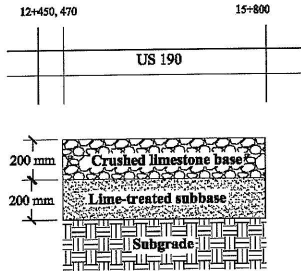
Figure 22 Layout and profile for sections at highway US 190
