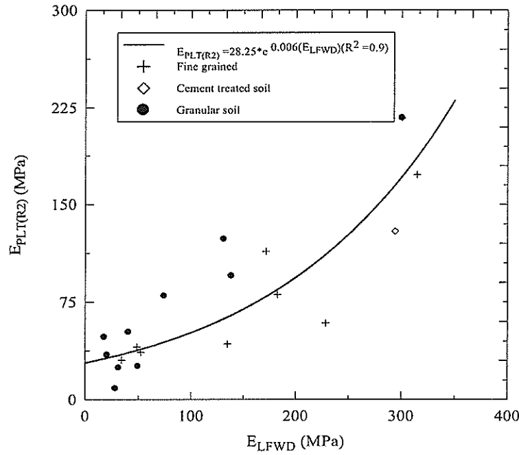
Figure 75 Correlation between E_{LFWD} and the E_{PLT(R2)} (laboratory test)
