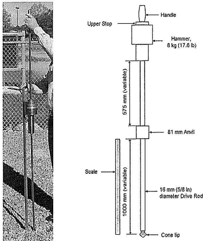
Figure 2 Dynamic Cone Penetrometer (DCP)
