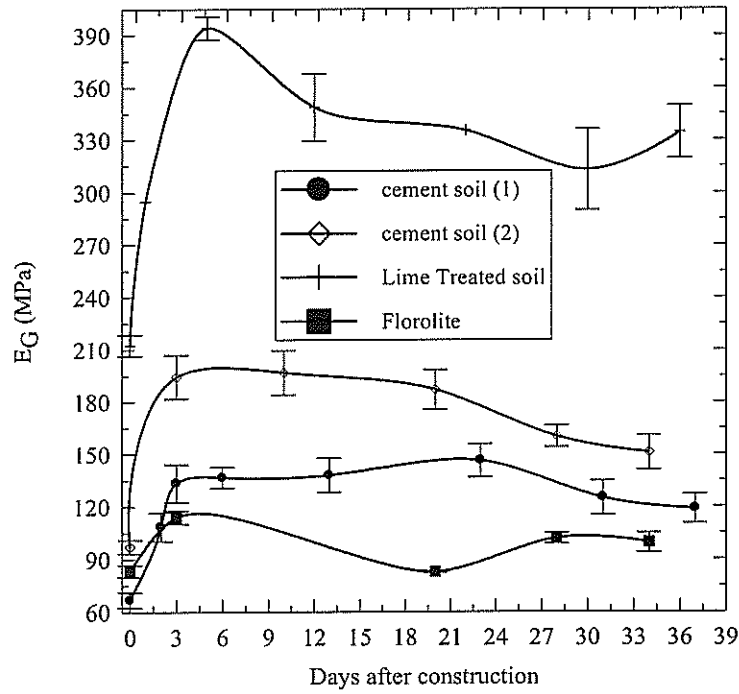
Figure 51 Geogauge modulus variations with time
