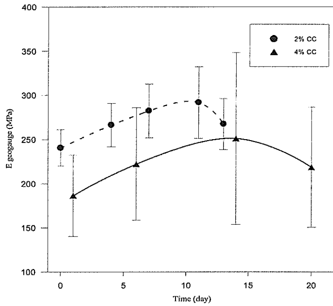
Figure 39 E_G with time for cement-soil
