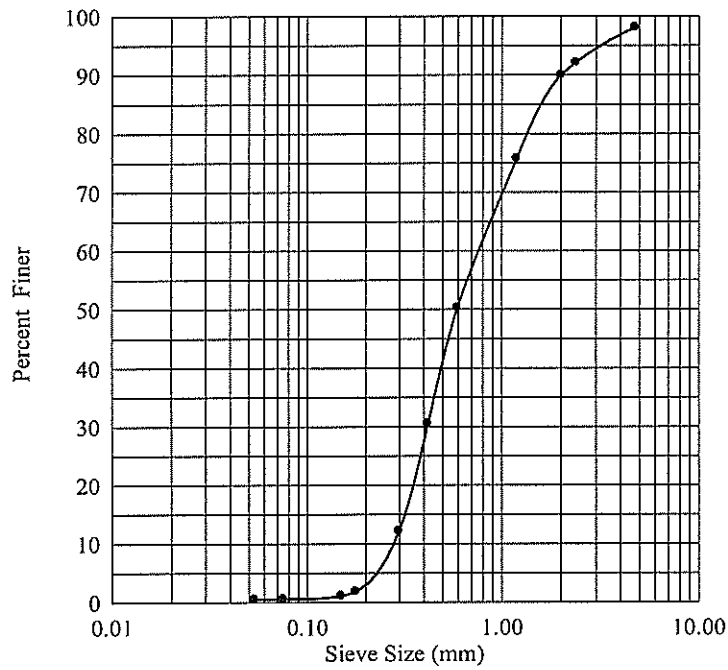
Figure 36 Gradation of sand
