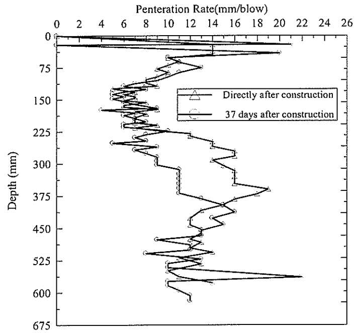
Figure 58 DCP-PR with time for BCS section
