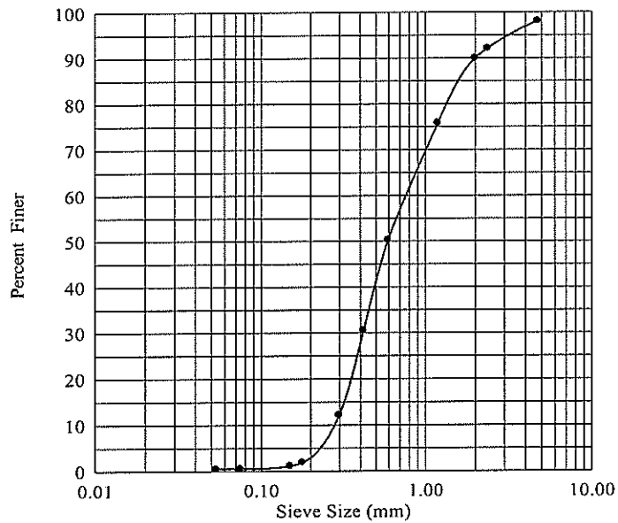
Figure 37 Gradation of RAP
