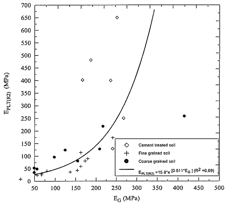
Figure 66 Correlation between E_G and the E_{PLT(R2)} (laboratory test)
