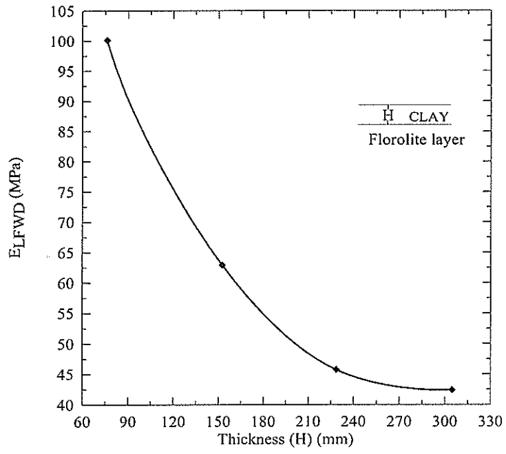
Figure 48 LFWD stiffness modulus curve for clay layer versus thickness
