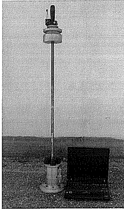
Figure 3 Prima 100 Light Falling Weight Deflectometer
