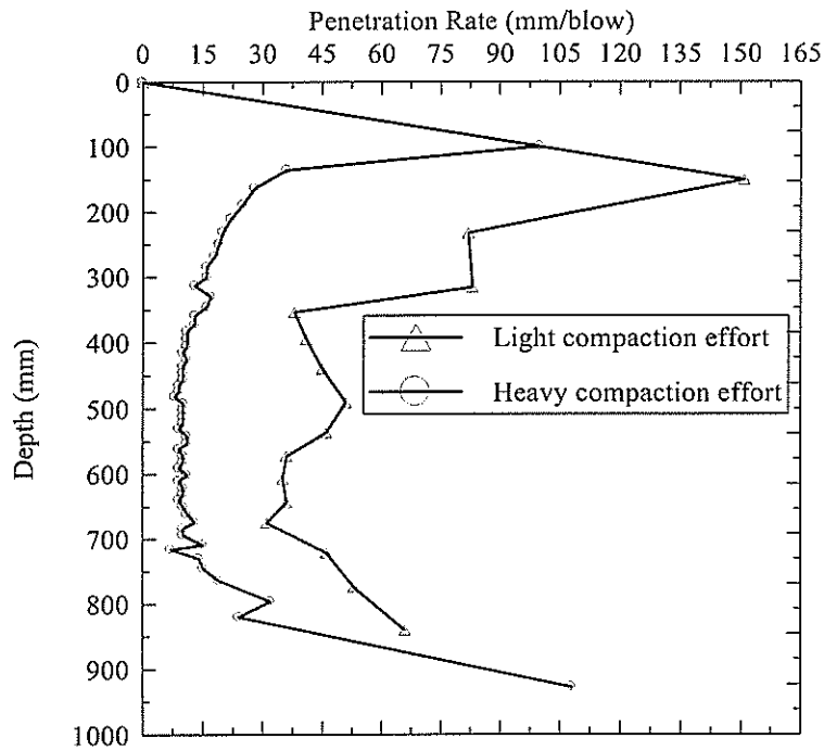
Figure 63 DCP-PR profiles for sand trench sections
