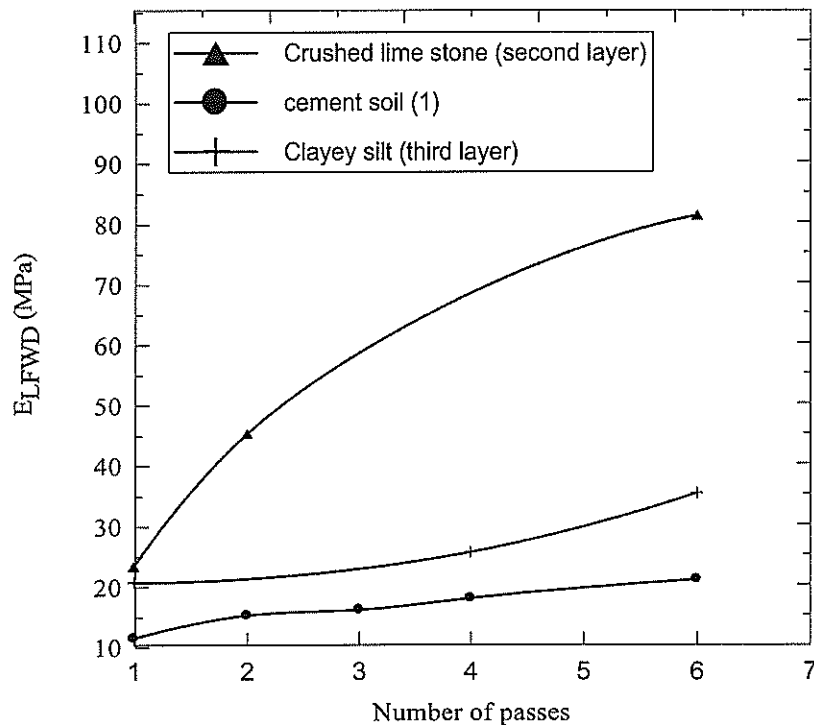
Figure 53 E LFW D variation with number of passes
