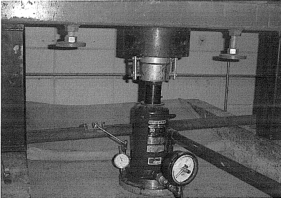
Figure 15 Plate Load Test setup
