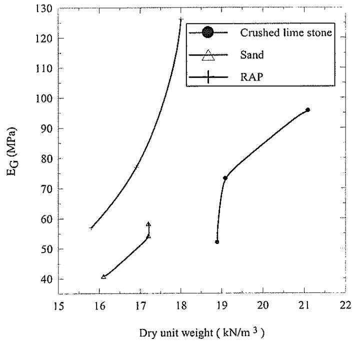
Figure 59 E_G and dry unit weight for different trenches
