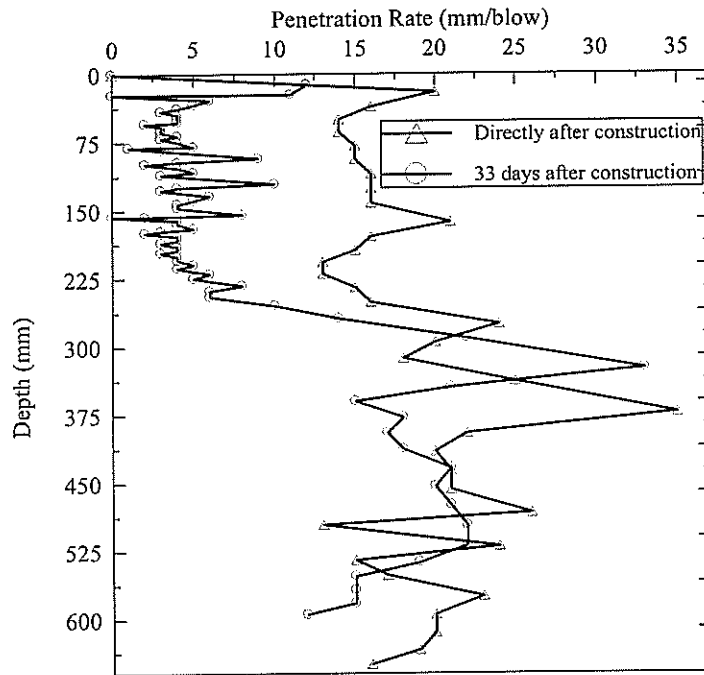
Figure 56 DCP-PR with time for cement soil section (2)
