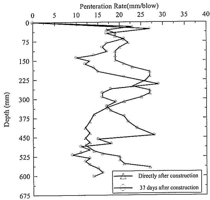
Figure 57 DCP-PR with time for lime-treated soil section
