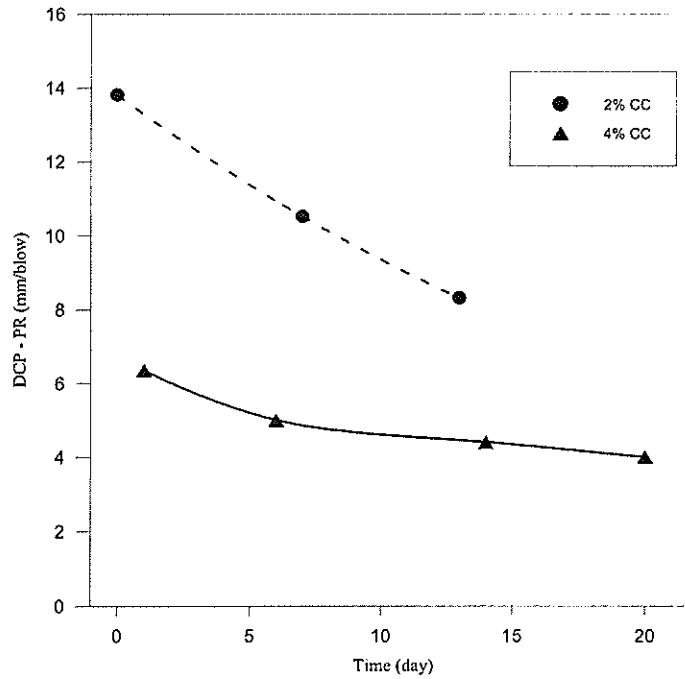
Figure 40 DCP average PR (8 inch) with time for cement-soil
