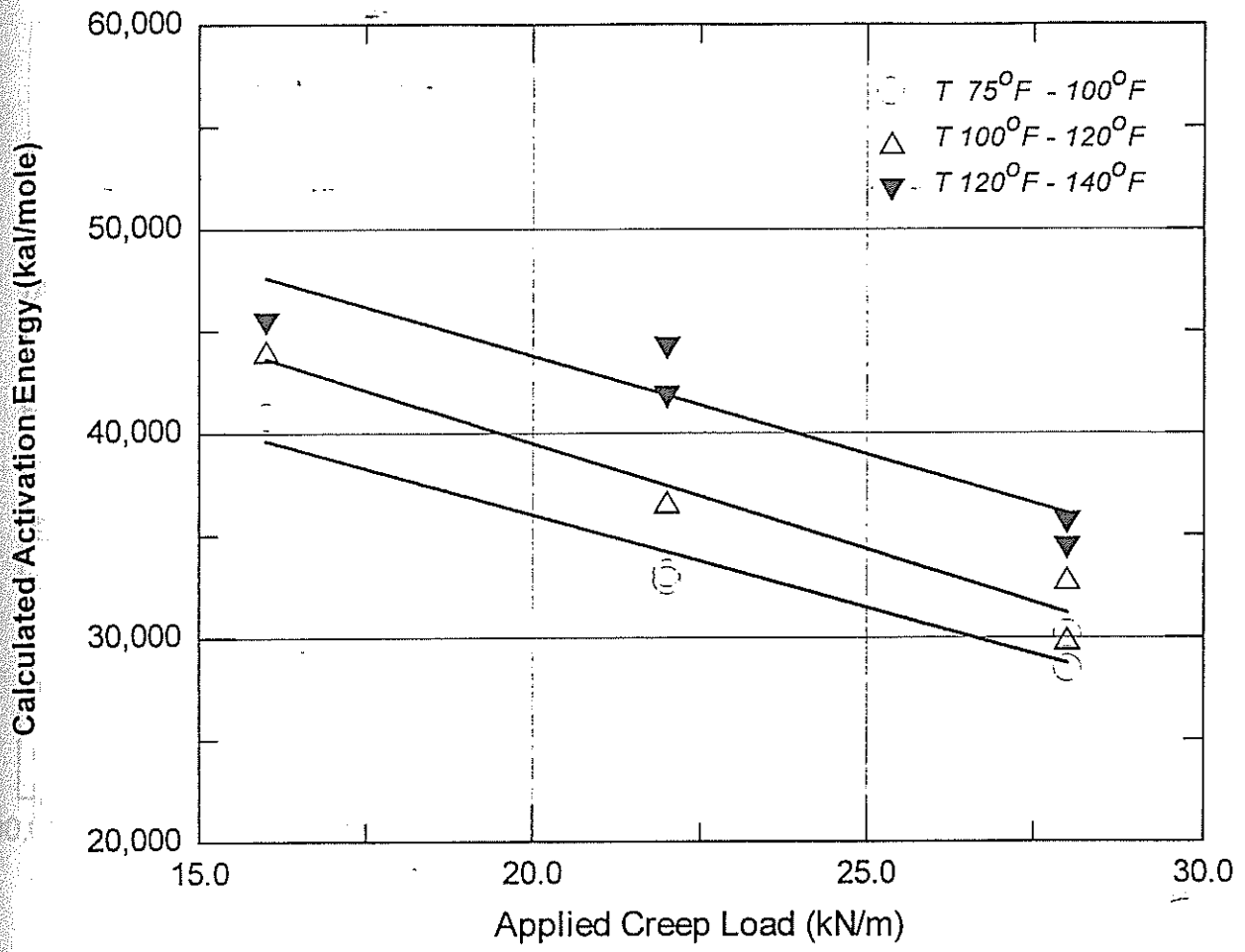
Figure 32 Estimation of E at various creep loads
