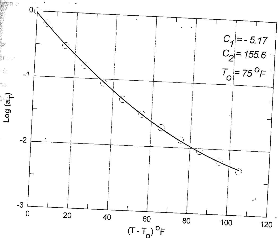
Figure 44 Analytical values of a_T for the HDPE geogrid
