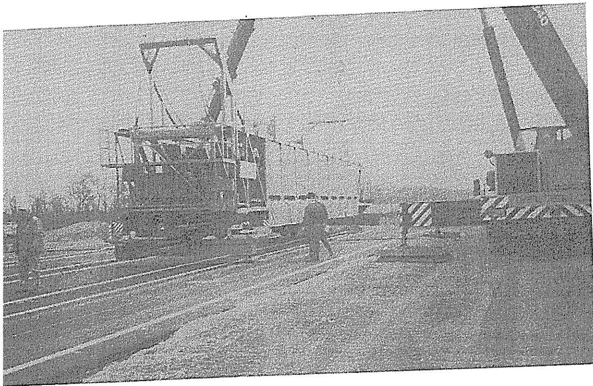
Moving the Accelerated Loading Facility (ALF)
