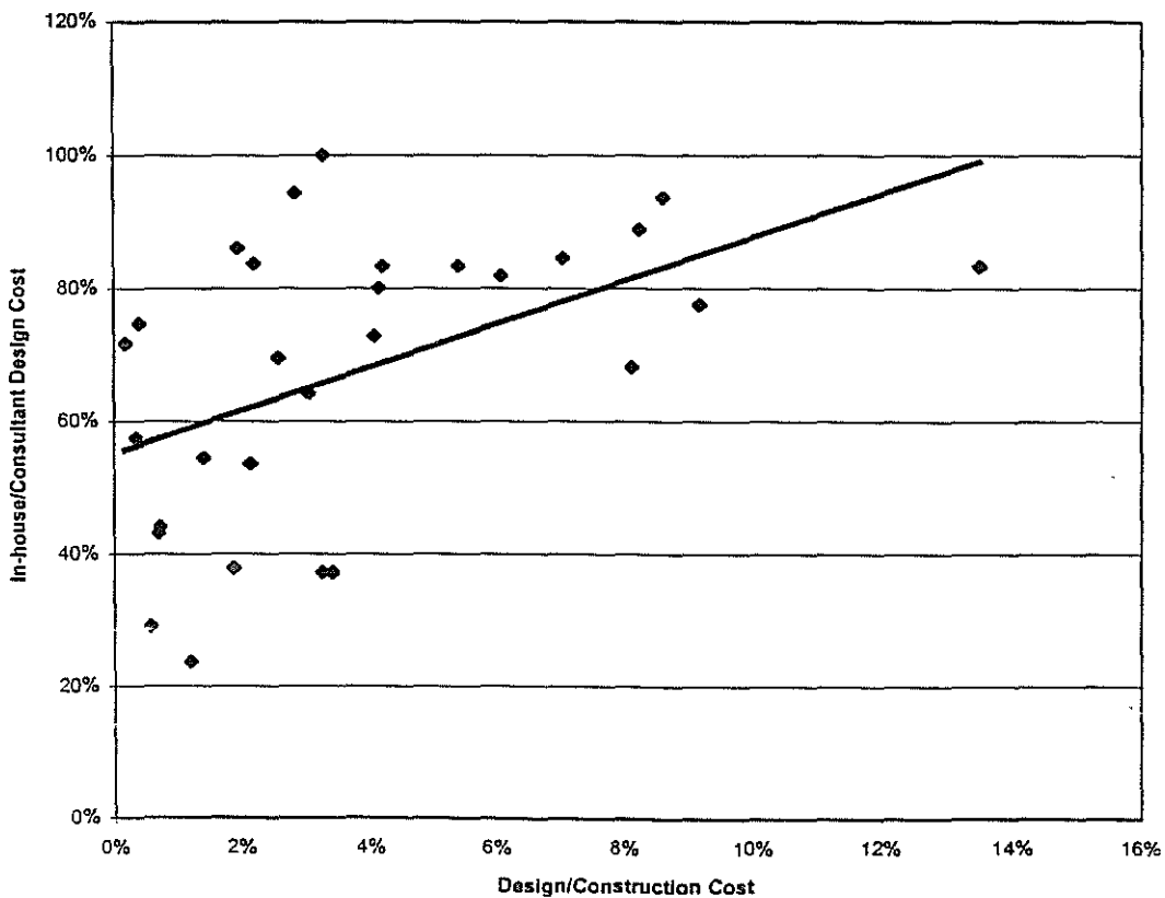
Figure 6.4: In-house/Consultant Design Cost versus Design/Construction Cost
